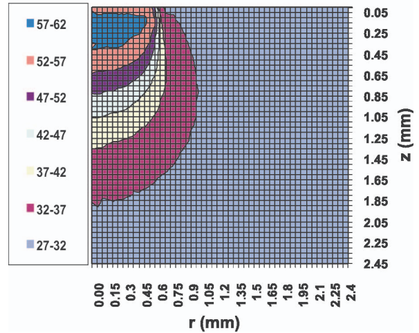
Fig. 5 Computed in-depth temperature distribution in both radial and axial directions at the end of laser pulse (350 \mu\text{s} ): a pulse energy 1.1 J; wavelength 1314 nm; spot diameter 1.3 mm.
