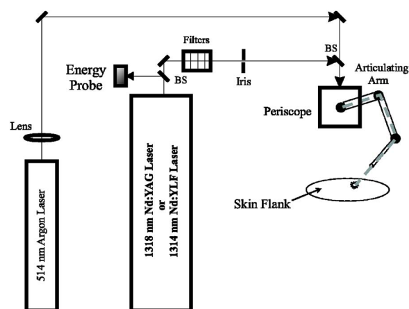
Fig. 3 Experimental setup for nanosecond experiment.
