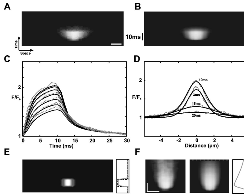
Fig. 4 Reconstruction of microscopic \text{Ca}^{2+} release fluxes. (a) Line scan image of an artificial \text{Ca}^{2+} spark generated by TFPF of the \text{Ca}^{2+} cage DM-Nitrophen using a flash that lasted 10 ms. The image shows the increase in fluo-3 fluorescence in response to the uncaging flash. Scale bar: 2 \mu\text{m} . (b) The best-fit simulated line scan image that was calculated using a model of \text{Ca}^{2+} and fluo-3 movements and binding. (c) In this graph the time courses of normalized fluorescence recorded at various locations of the artificial spark (dashed lines) are compared with the corresponding time courses of the “best fit” model calculation (solid lines). (d) Comparison of fluorescence profiles extracted from experimental data (dashed) and fit (solid). (e) This image shows the distribution of \text{Ca}^{2+} release flux underlying the simulation that best fit the experimental data. The graph next to the image compares the estimated time course of release (gray) with the flash time course. (f) The fitting approach validated using TFPF [(a) to (e)] was applied to an average \text{Ca}^{2+} spark recorded in an intact heart cell loaded with the indicator fluo-4. The average spark is shown next to the fitted spark. The time course of \text{Ca}^{2+} release underlying the fitted spark is shown on the right. Scale bars: 2 \mu\text{m} , 10 ms.
