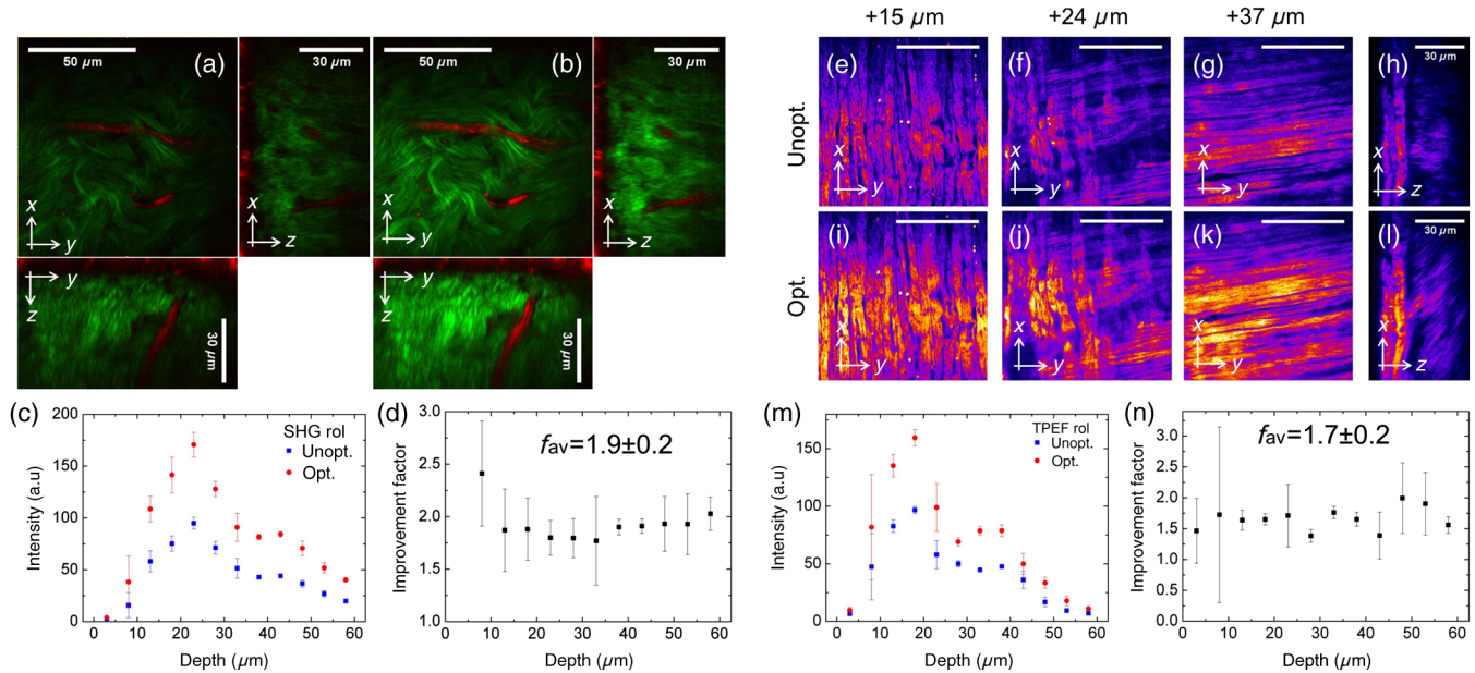
Fig. 3 Ex-vivo Lifestact mouse skin imaged at a depth of 30\ \mu\text{m} (a) without and (b) with aberration correction. Green channel: SHG emitted by collagen; Red channel: TPEF emitted by vasculature. (c) SHG signal within a central Rol with depth. The data was binned over 5\ \mu\text{m} to display an average signal intensity and error bars given by a standard deviation. (d) Calculated signal improvement factors. (e to l) Lifestact mouse intestine showing orthogonally oriented layers of smooth muscle imaged without and with aberration correction. The first slice of the stack lay \approx 70\text{-}\mu\text{m} deep within the tissue. The three depths presented were measured with respect to the start of the image stack. Scale bar: 50\ \mu\text{m} , false colour scale applied for clarity. (m) TPEF signal (red channel) within a small, central Rol with depth, and (n) calculated signal improvement factors.
