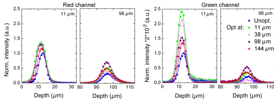
Fig. 5 Axial intensity profiles of multiply dye-stained beads at depths of 11 and 98 \mu\text{m} with all DMM shapes in the look-up table for the red and green channel. The intensity in each channel was normalised to unity for the unoptimized DMM shape for the bead at the shallowest depth of 11 \mu\text{m} . The intensity in the green channel was scaled to the intensity in the red channel by renormalisation of the y-axis. Table 1 lists the amplitude of the Gaussian fits A to the intensity profiles and the calculated improvement factors f . The first column indicates the time difference \Delta in days between the acquisition of the optimization and the image.
