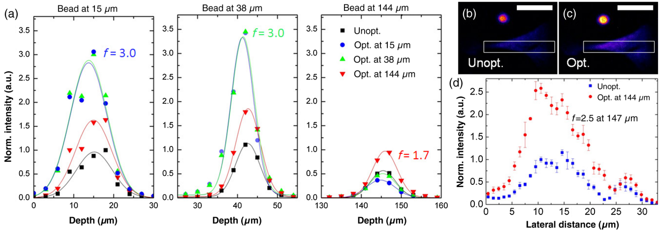
Fig. 4 (a) Axial intensity profiles through beads at the depths of 15, 38, and 144 \mu\text{m} embedded within the organotypic tissue culture. (b) to (c) Detail showing the bead and adjacent cells at a depth of 144 \mu\text{m} without and with correction in the red channel (false colour scale applied for clarity). Scale bar: 15 \mu\text{m} . (d) Lateral intensity profile (binned over 1 \mu\text{m} , error bars: one standard deviation) within the indicated Rol.
