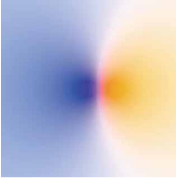
Figure 2.12 Universal color pattern near an isolated phase singularity.
