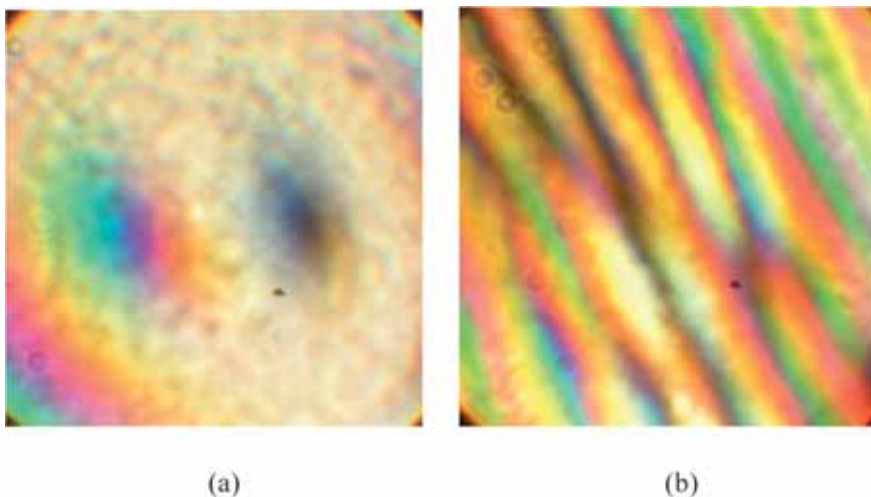
Figure 2.11 Singularity obtained in (a) white-light beam passing a double-axial crystal placed between matched polarizer and analyzer: (a) without a reference wave and (b) with a reference wave. (Figure continued on next page.)
