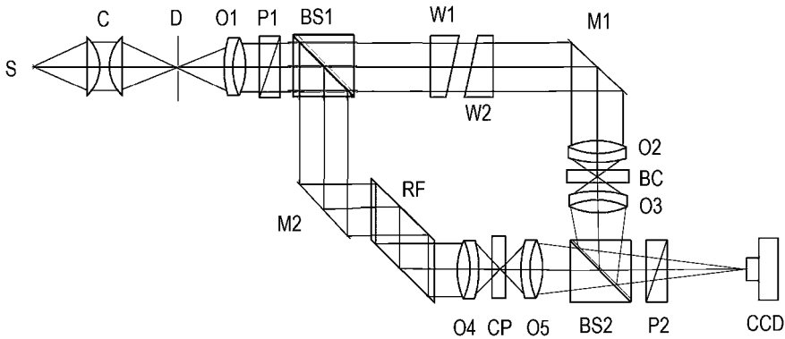
Figure 2.10 Experimental arrangement. S: white light source; C: condenser; D: 20 \mu\text{m} diameter diaphragm; O1 ( f = 200 mm), O2, O3, and O4: objectives; P1 and P2: polarizer and analyzer; BS1 and BS2: beam-splitting cubes; M1 and M2: mirrors; BC: singularity-generating object; CP: compensating plate; RF: Fresnel rhombus; W1 and W2: moving and stationary optical wedges; CCD: camera.
